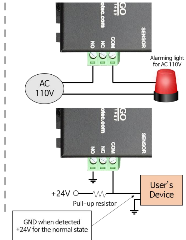
- Connection examples
